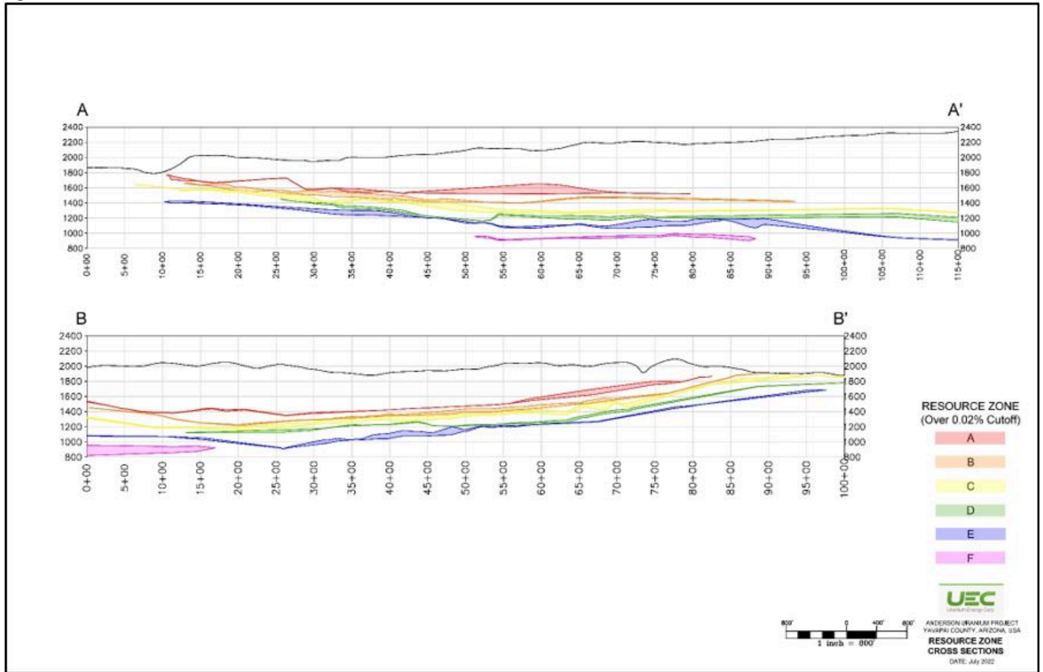
Figure 6-4: Cross Sections
